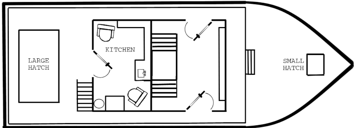
FIRST DECK
